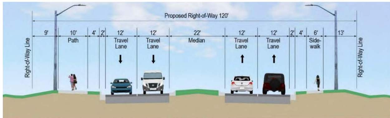
TYPICAL SECTION Avalon Road Four-Lane Divided Section
